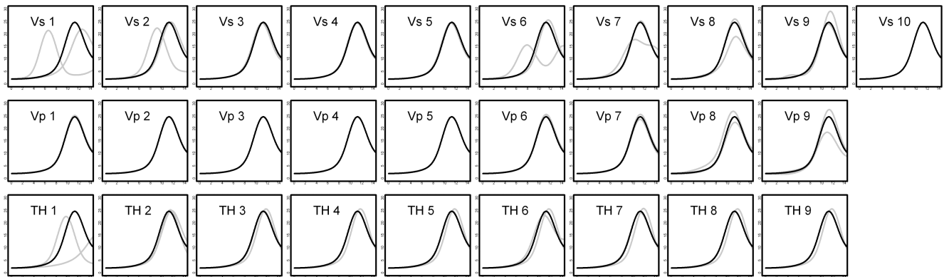
Fig. 3. Variations of theoretical H/V ratio for observation site KYT008 when changing a single parameter (S-wave velocity, P-wave velocity or thickness of each layer) at once.
